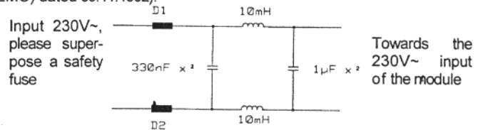
D1/D2 = 6-hole-VHF-wide band choke
